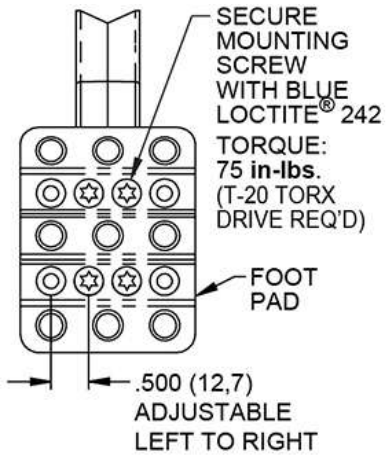
FOOT PAD DETAIL
