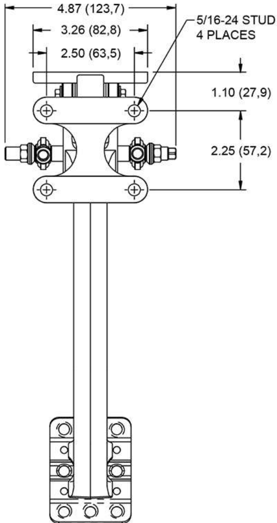
FOOT PAD DETAIL
